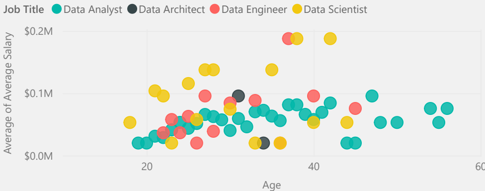
Age vs Average Salary
