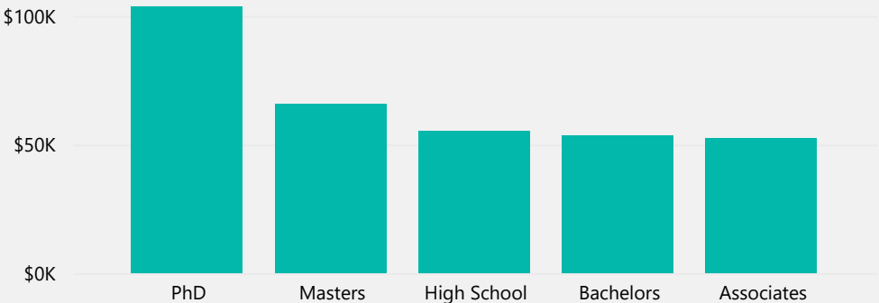
Average Salary by Education Level
