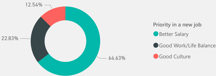
Most Important Factors in a New Job
