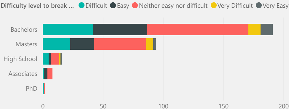
Difficulty Breaking Into Data by Education
